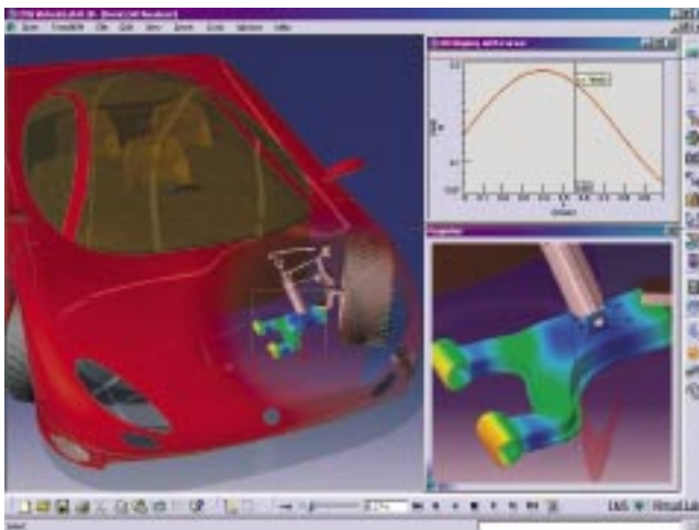
Virtual.Lab's flexible body analysis calculates the critical bending of each component, such as the arm in a front suspension unit as shown above. During an animation of the unit's movement, graphs are synchronized with the geometry display, giving you even more insight into the dynamics of a given maneuver.
