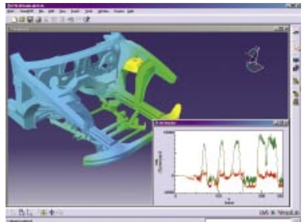
Apply measured loads to the model of a vehicle front section to predict fatigue life - and detect the most critical locations.
